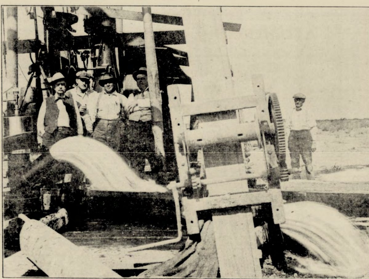
THE FIRST PUMPED IRRIGATION WELL IN LEON VALLEY—PUMPING OVER 1000 GALLONS OF WATER A MINUTE
